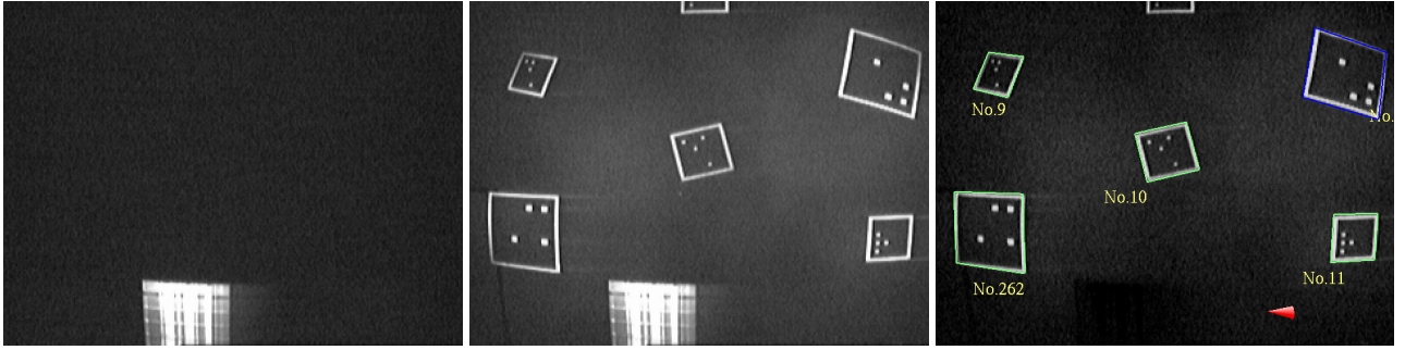
(a) Captured images when infrared LEDs are switch-off. (b) Captured images when infrared LEDs are switch-on. (c) Results of marker recognition.
