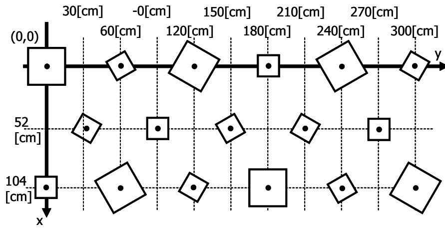
Figure 9. Layout of markers.
