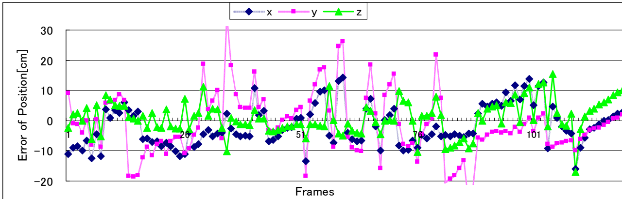
Figure 11. Error of estimated camera position.
