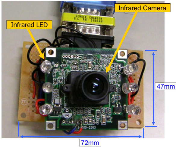
Figure 5. Infrared camera and infrared LEDs.
