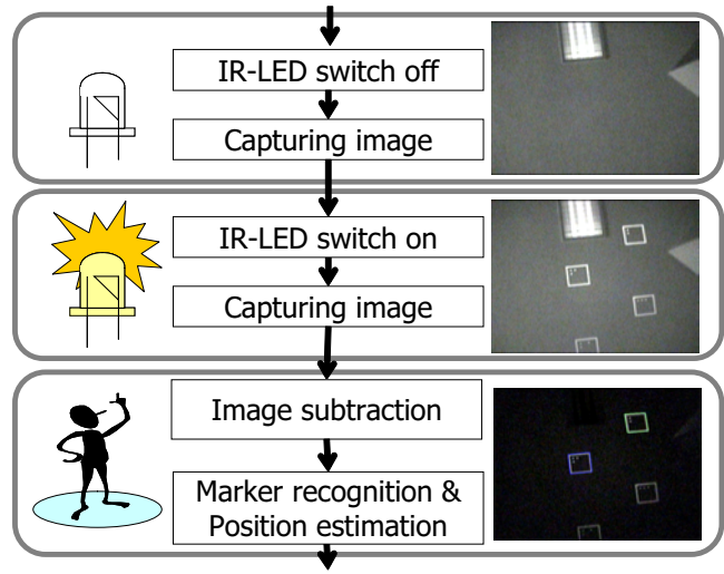
Figure 6. Flow diagram of capturing markers.
