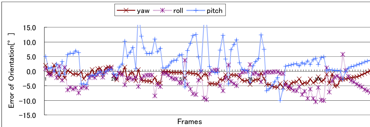
Figure 12. Error of estimated camera orientation.
