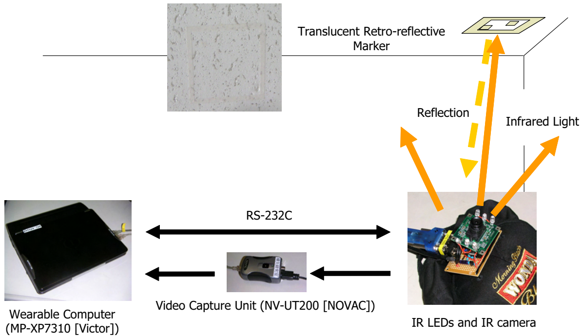
Figure 4. Overview of localization system.
