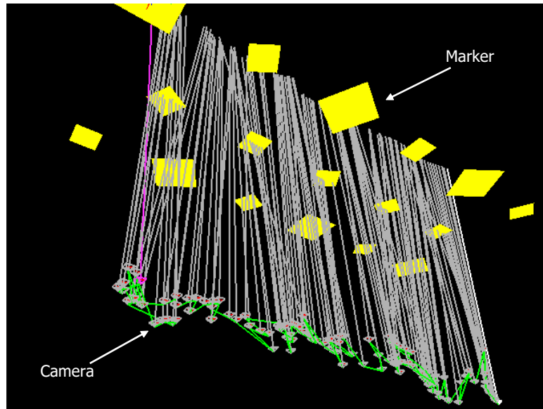
Figure 10. Estimated camera position and orientation.
