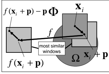
図3 エネルギー算出における画素の関係 Fig.3 Relationship between pixels in energy calculation.
