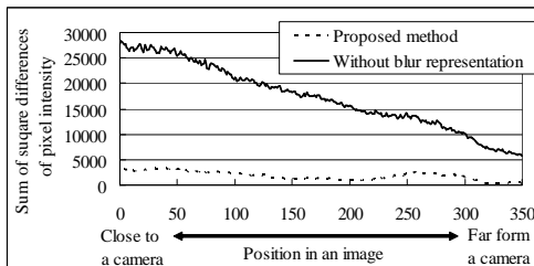
図 8 エッジ上の位置と輝度値の差の 2 乗和の関係 Fig. 8 Square differences of intensity between real and composed images
